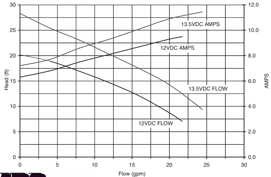
12V DC MOTOR FOR 24V DC AMPS DIVIDE 12V AMPS BY TWO
