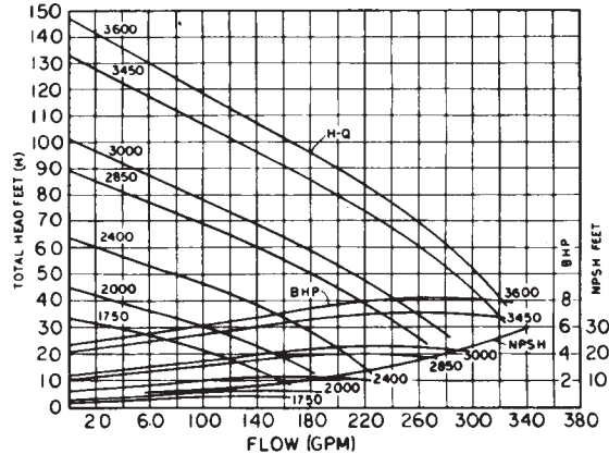
FLOMAX 15 - 3"
