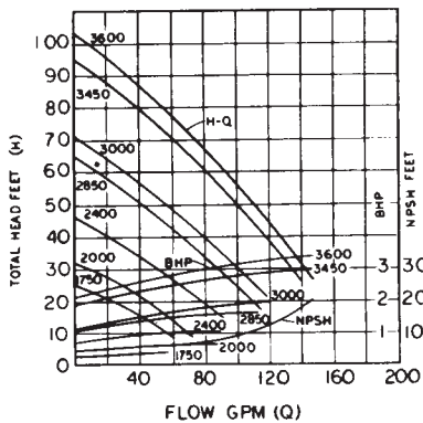
FLOMAX 8 - 2"
