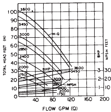
FLOMAX 5 - 1 1/2"
