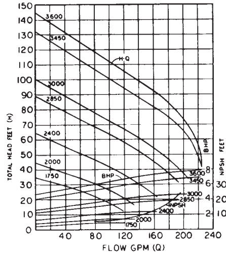
FLOMAX 15 - 3"
